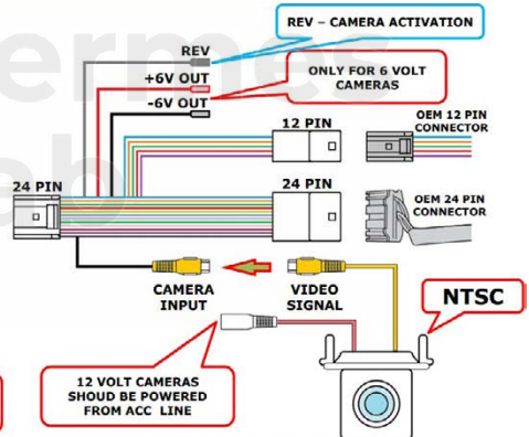
24 PIN SOCKET FOR REAR VIEW CAMERA CONNECTION
