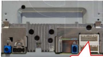
24 PIN SOCKET FOR REAR VIEW CAMERA CONNECTION
